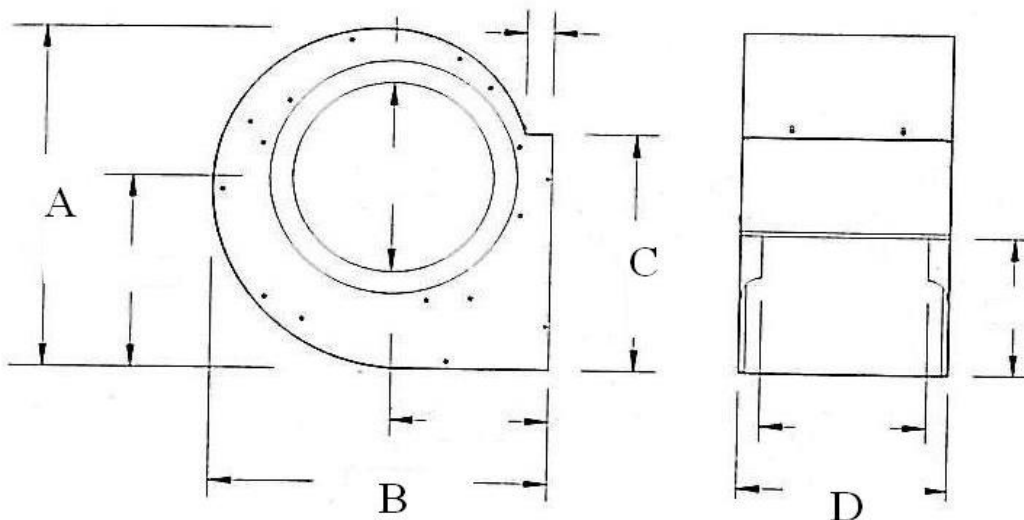
Housing Dimensions (in)
