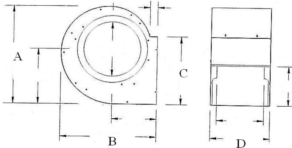
Housing Dimensions (in)
