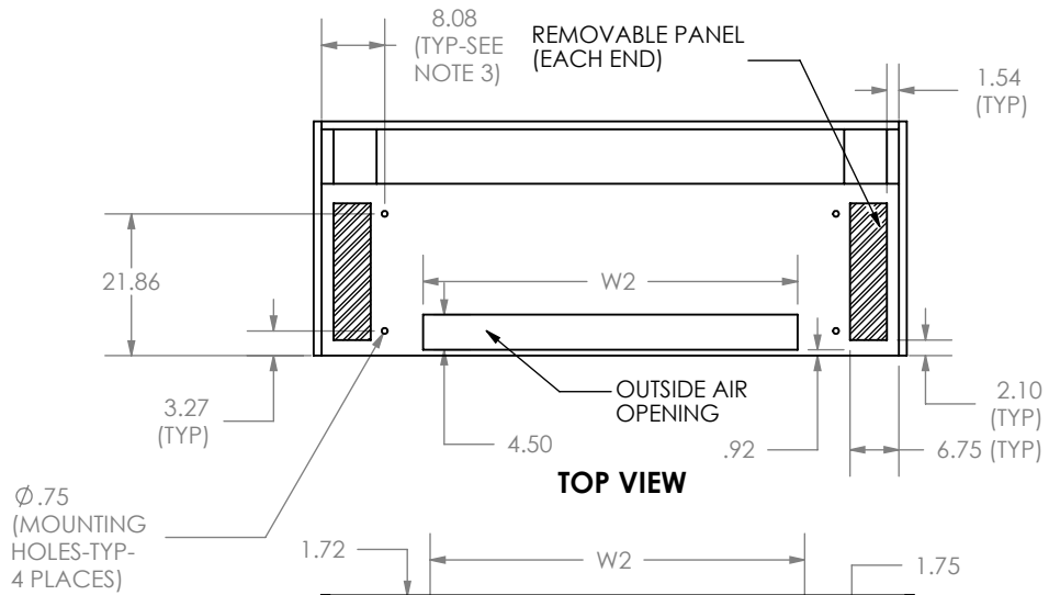
BOTTOM VIEW
