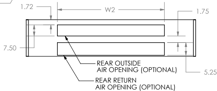
REAR VIEW
